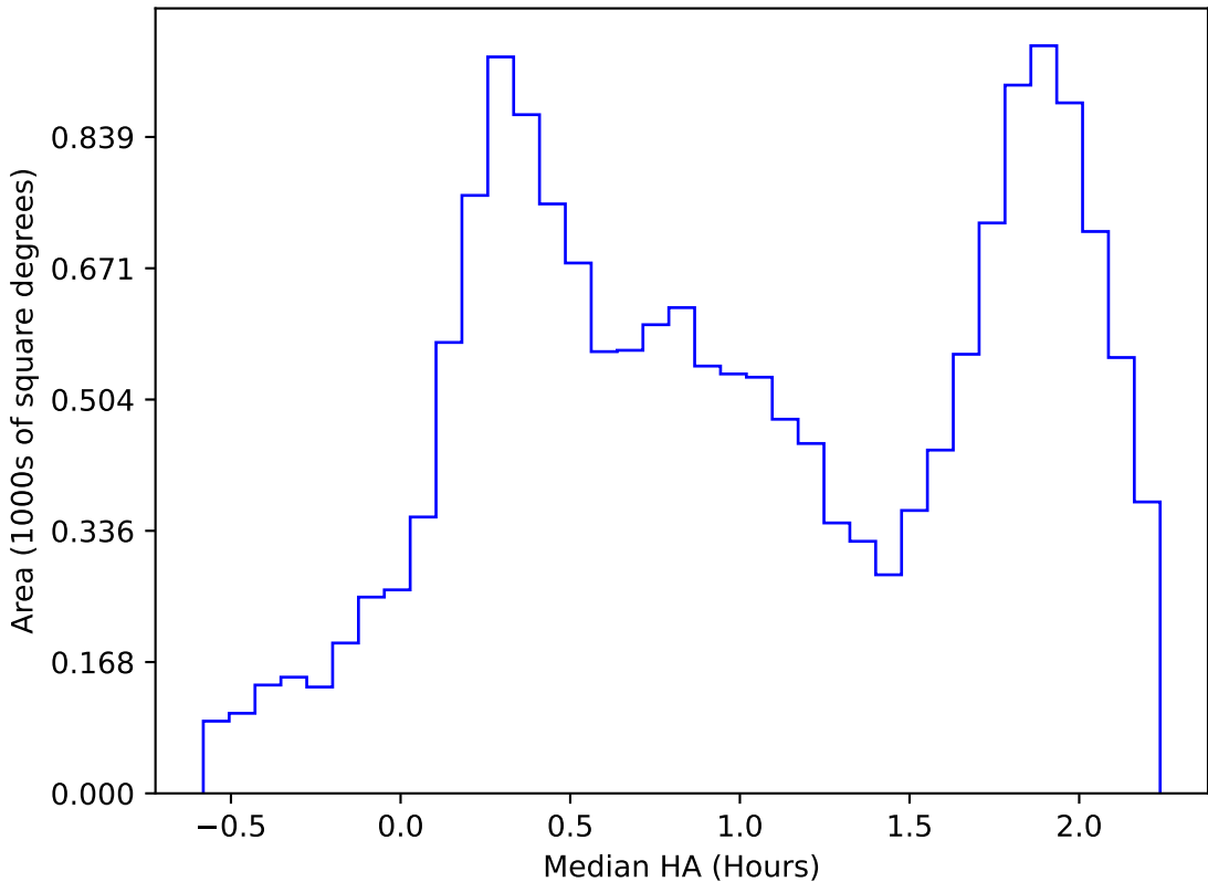
internal_u_expt27_nscale1.5v3.4_10yrs WFD i band: Median HA
