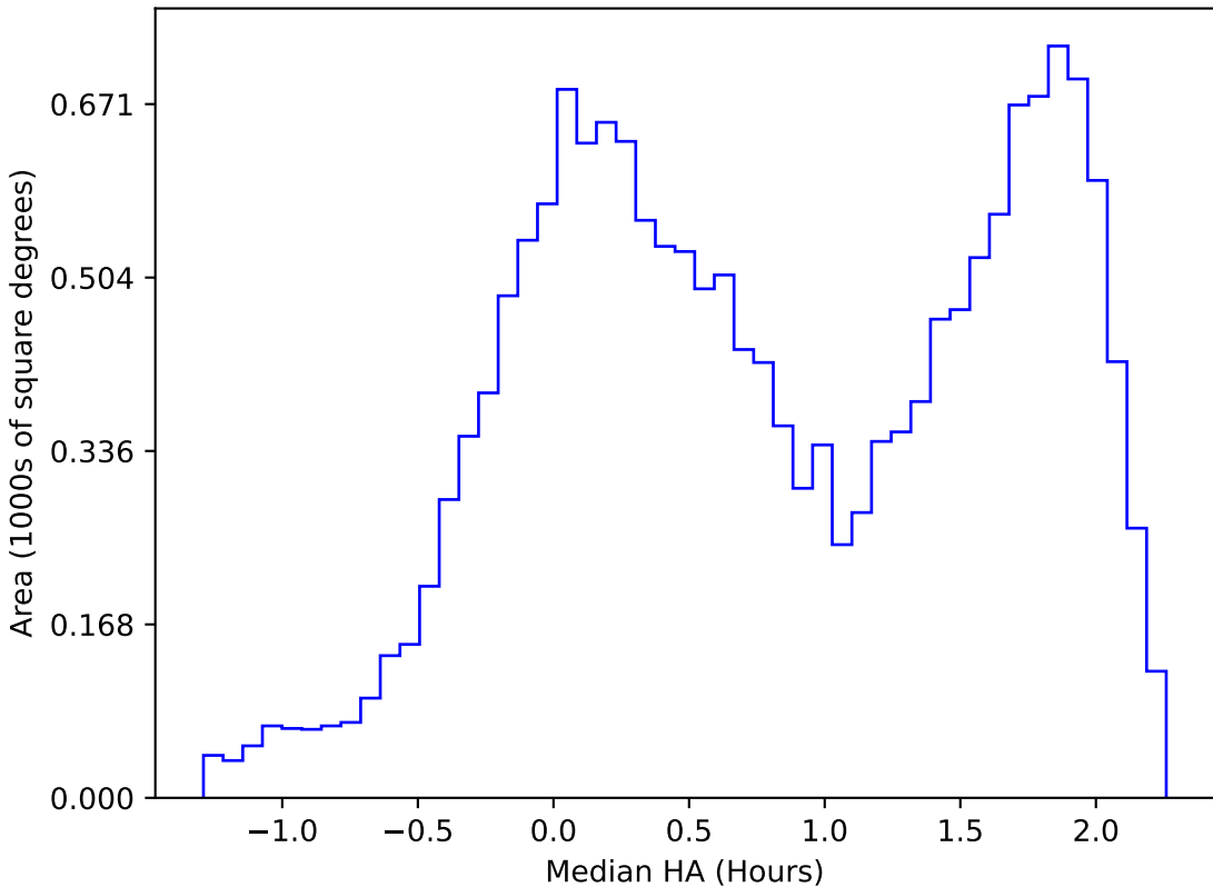
internal_u_expt27_nscale1.5v3.4_10yrs WFD g band: Median HA
