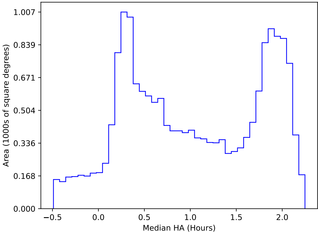
internal_u_expt27_nscale1.5v3.4_10yrs WFD all bands: Median HA
