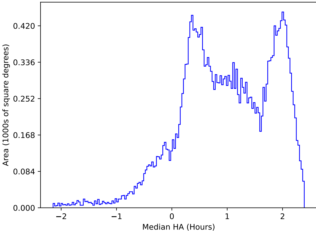
internal_u_expt27_nscale1.5v3.4_10yrs All sky z band: Median HA
