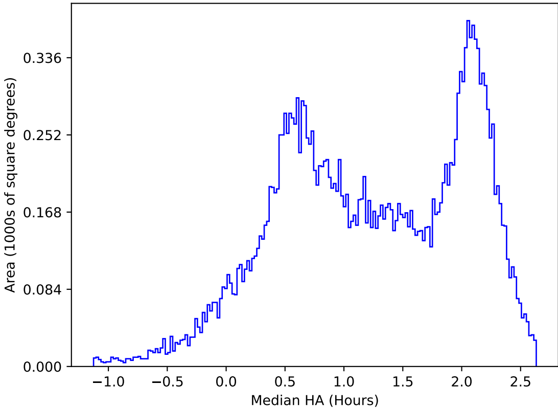
internal_u_expt27_nscale1.5v3.4_10yrs All sky y band: Median HA
