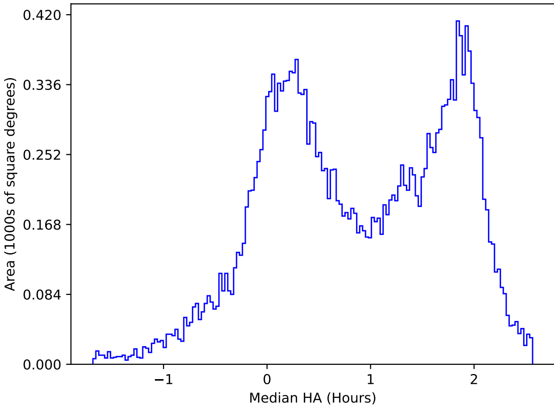
internal_u_expt27_nscale1.5v3.4_10yrs All sky u band: Median HA
