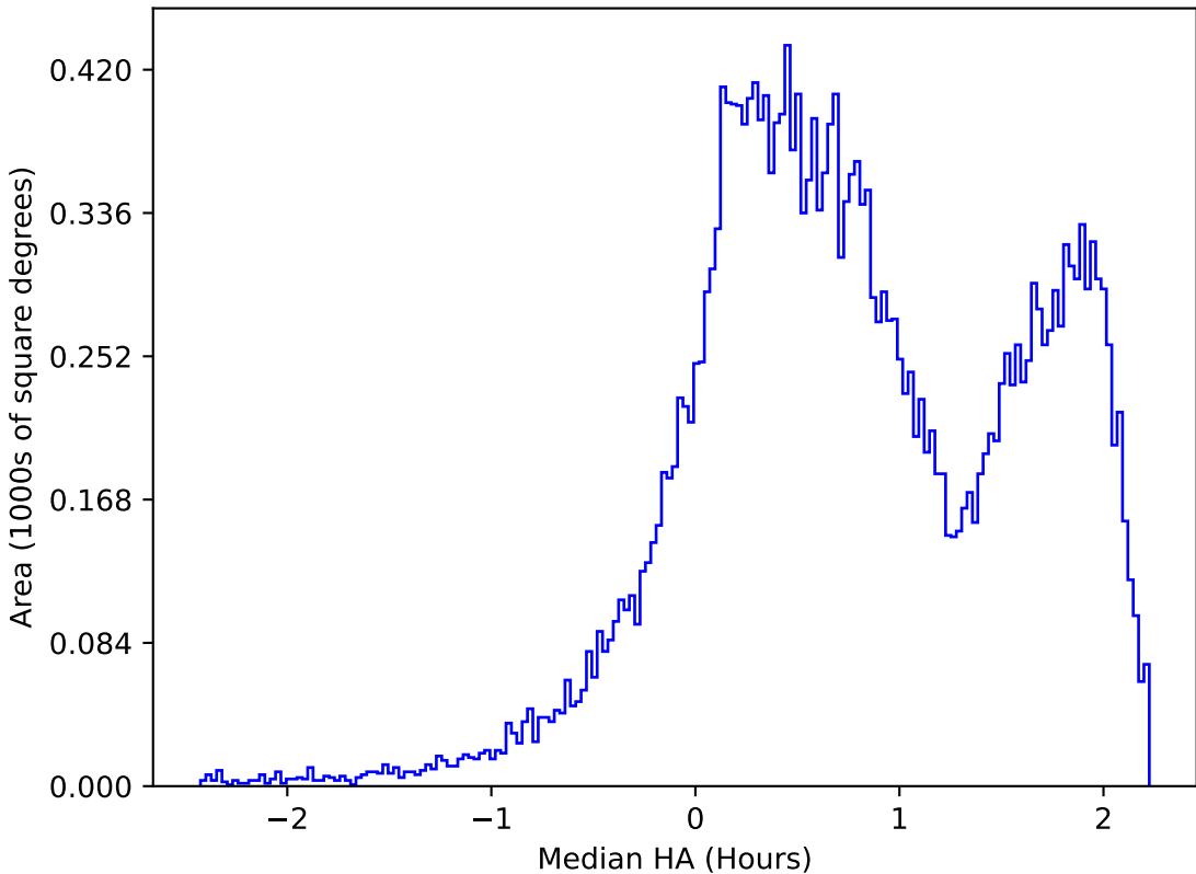
internal_u_expt27_nscale1.5v3.4_10yrs All sky r band: Median HA
