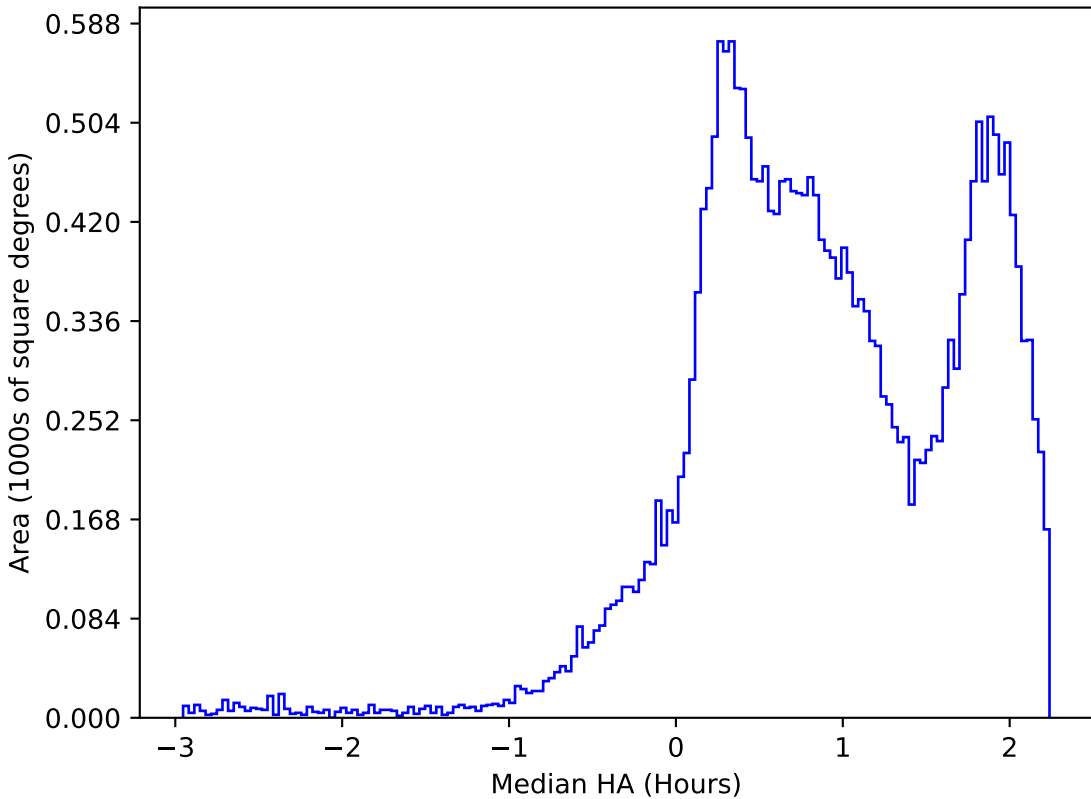
internal_u_expt27_nscale1.5v3.4_10yrs All sky i band: Median HA
