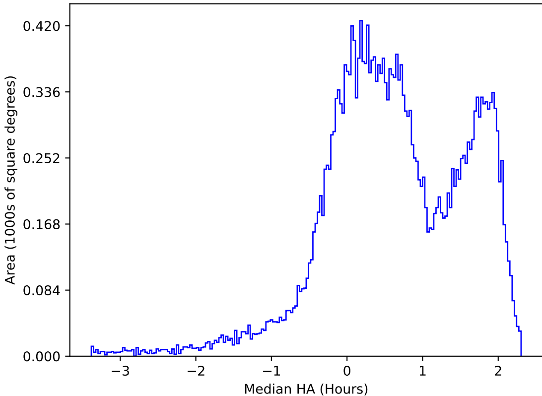
internal_u_expt27_nscale1.5v3.4_10yrs All sky g band: Median HA
