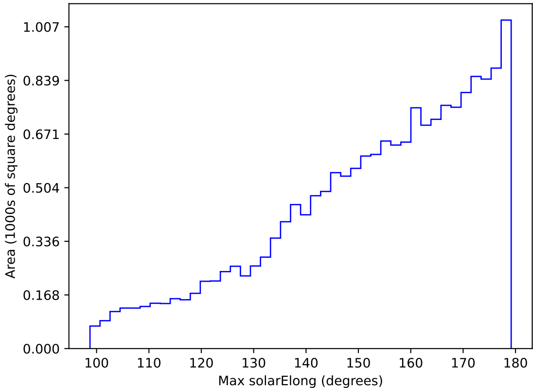
internal_u_expt27_nscale1.5v3.4_10yrs WFD y band: Max solarElong
