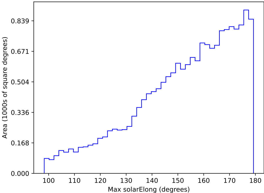
internal_u_expt27_nscale1.5v3.4_10yrs WFD u band: Max solarElong
