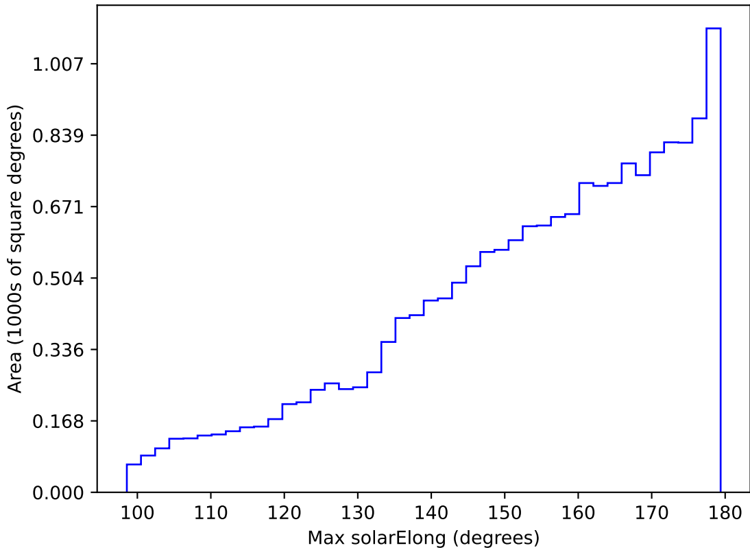
internal_u_expt27_nscale1.5v3.4_10yrs WFD i band: Max solarElong
