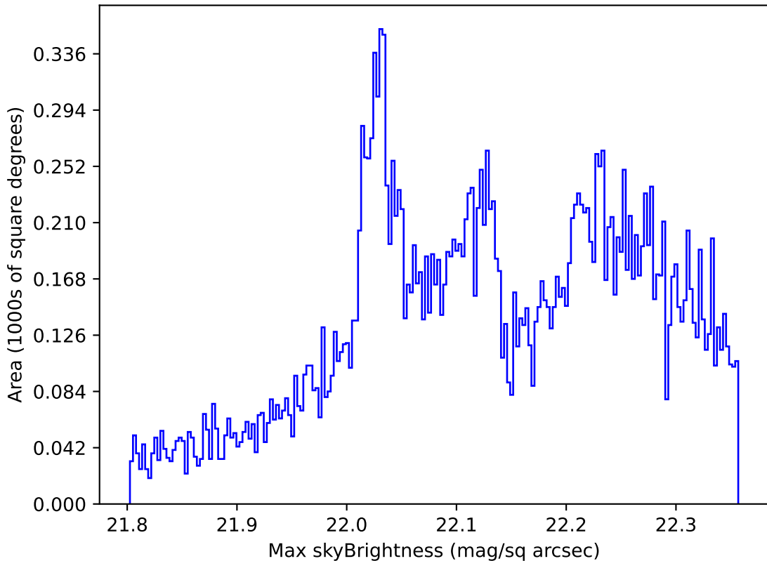
internal_u_expt27_nscale1.5v3.4_10yrs All sky g band: Max skyBrightness
