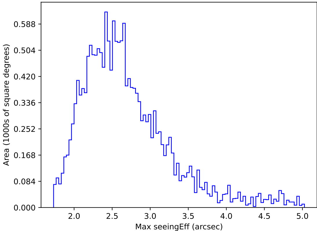
internal_u_expt27_nscale1.5v3.4_10yrs WFD i band: Max seeingEff
