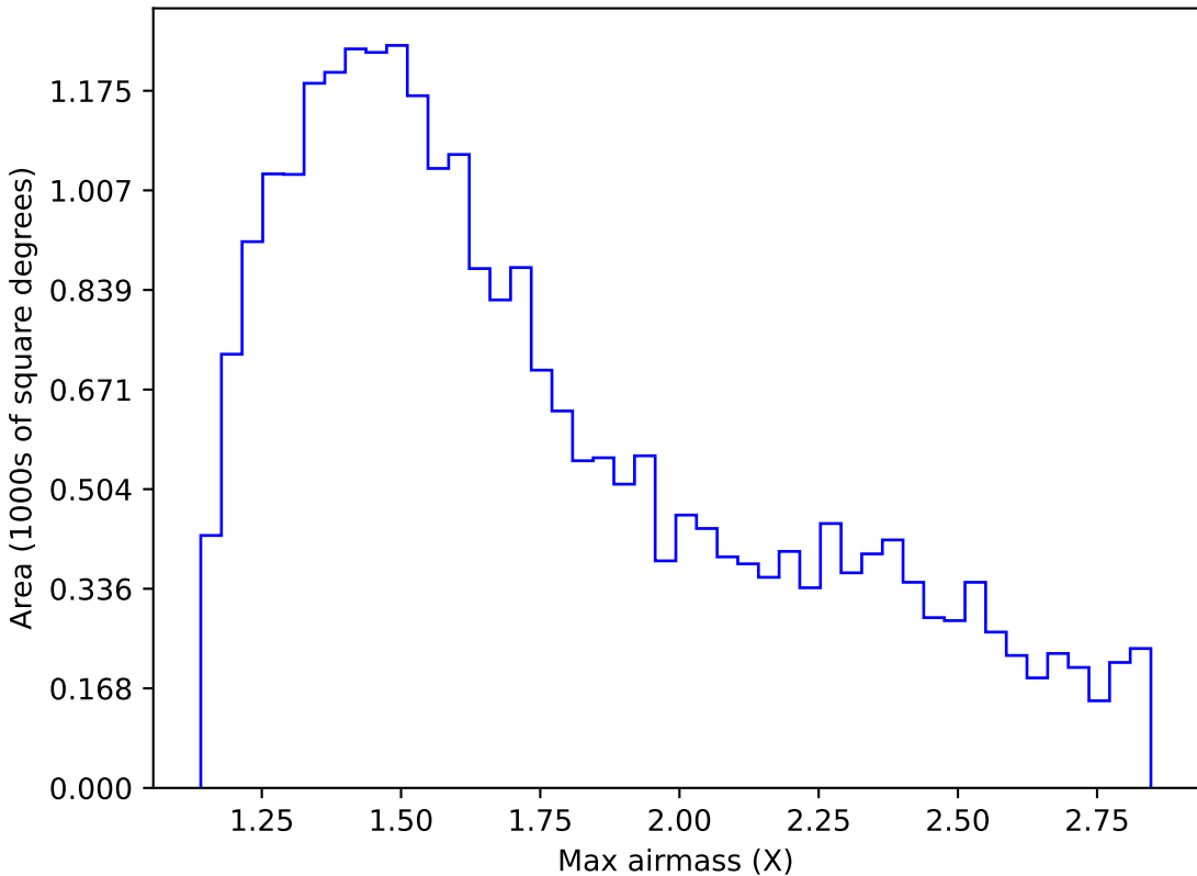
internal_u_expt27_nscale1.5v3.4_10yrs Yr 1 z band: Max airmass
