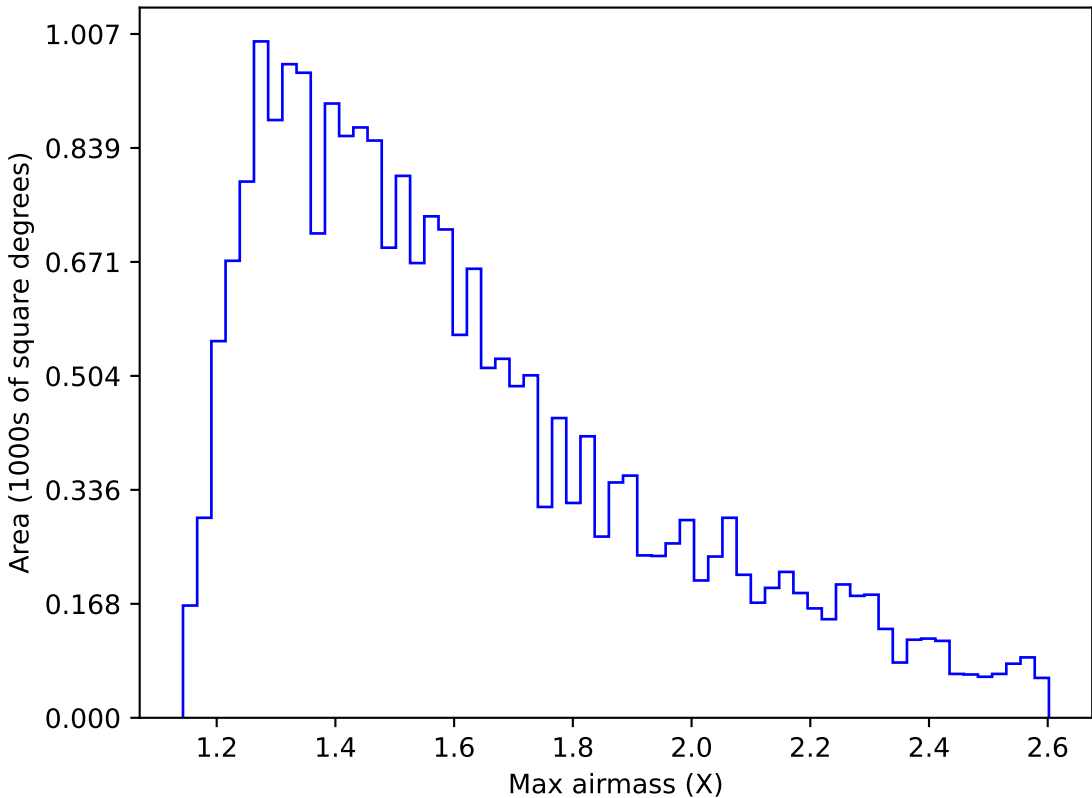
internal_u_expt27_nscale1.5v3.4_10yrs Yr 1 y band: Max airmass
