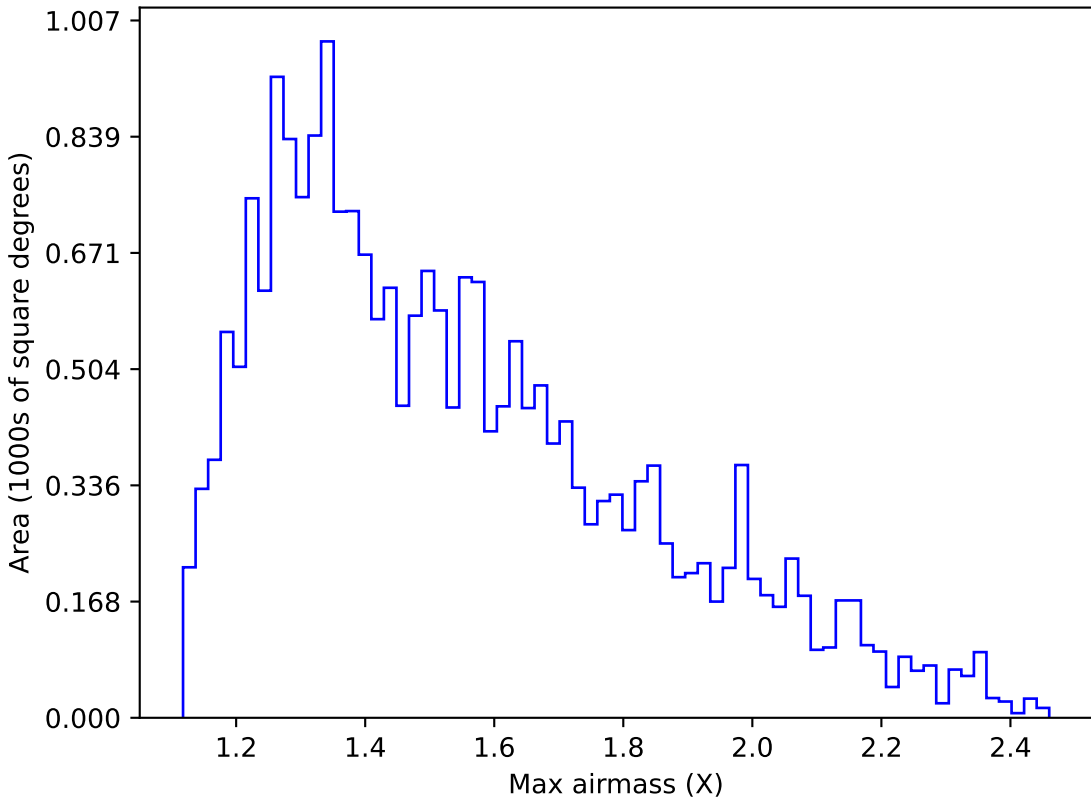
internal_u_expt27_nscale1.5v3.4_10yrs Yr 1 u band: Max airmass
