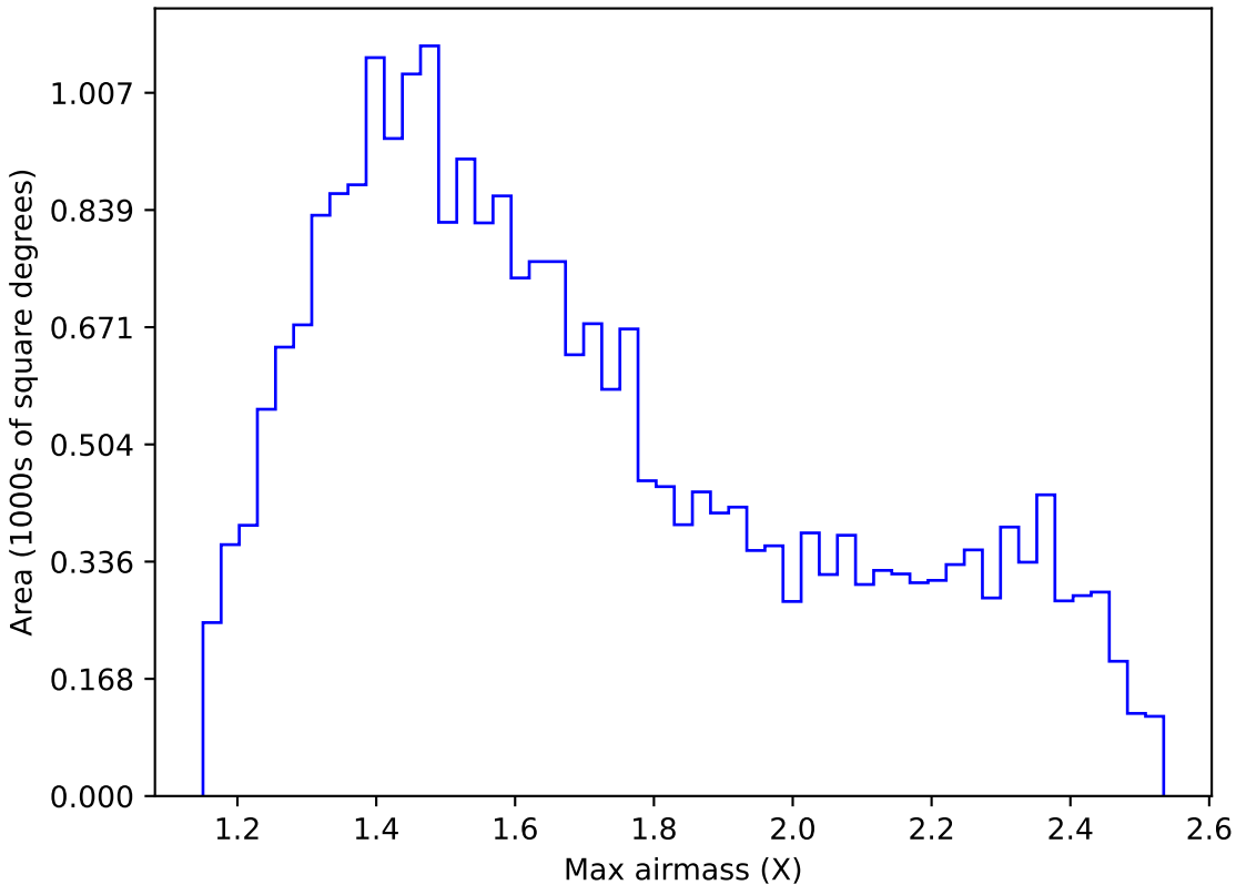
internal_u_expt27_nscale1.5v3.4_10yrs Yr 1 r band: Max airmass
