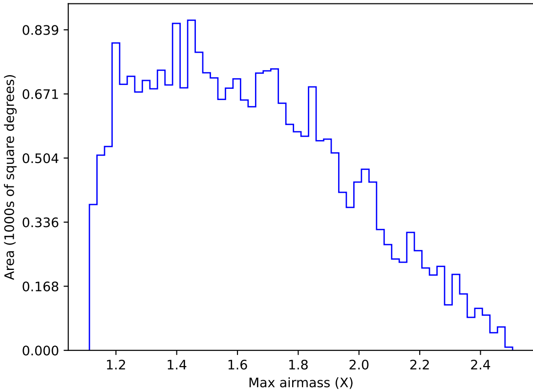
internal_u_expt27_nscale1.5v3.4_10yrs Yr 1 g band: Max airmass
