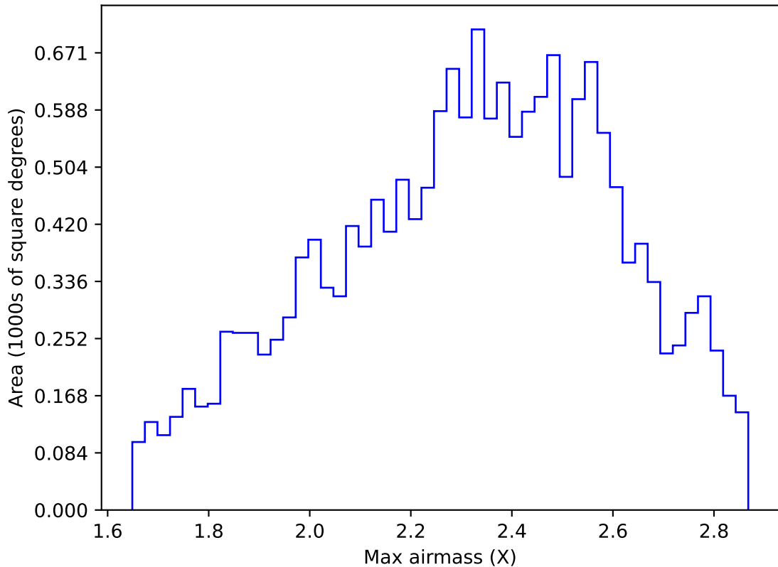
internal_u_expt27_nscale1.5v3.4_10yrs WFD y band: Max airmass
