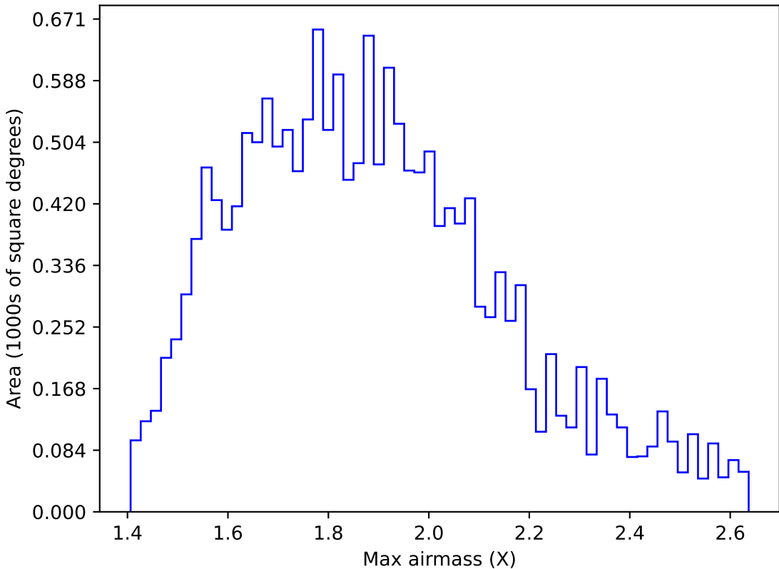
internal_u_expt27_nscale1.5v3.4_10yrs WFD u band: Max airmass
