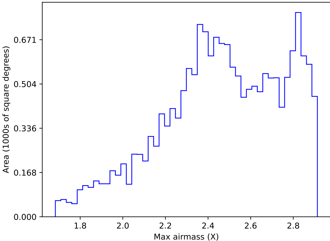
internal_u_expt27_nscale1.5v3.4_10yrs WFD i band: Max airmass
