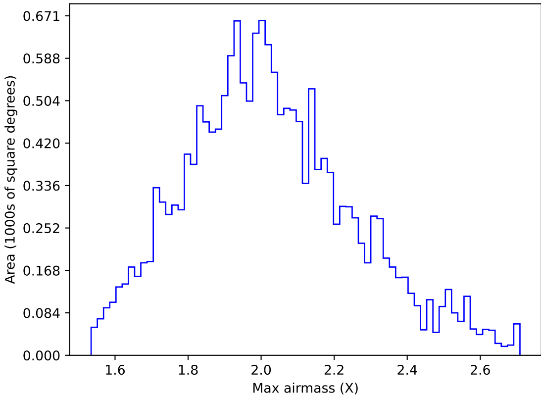
internal_u_expt27_nscale1.5v3.4_10yrs WFD g band: Max airmass
