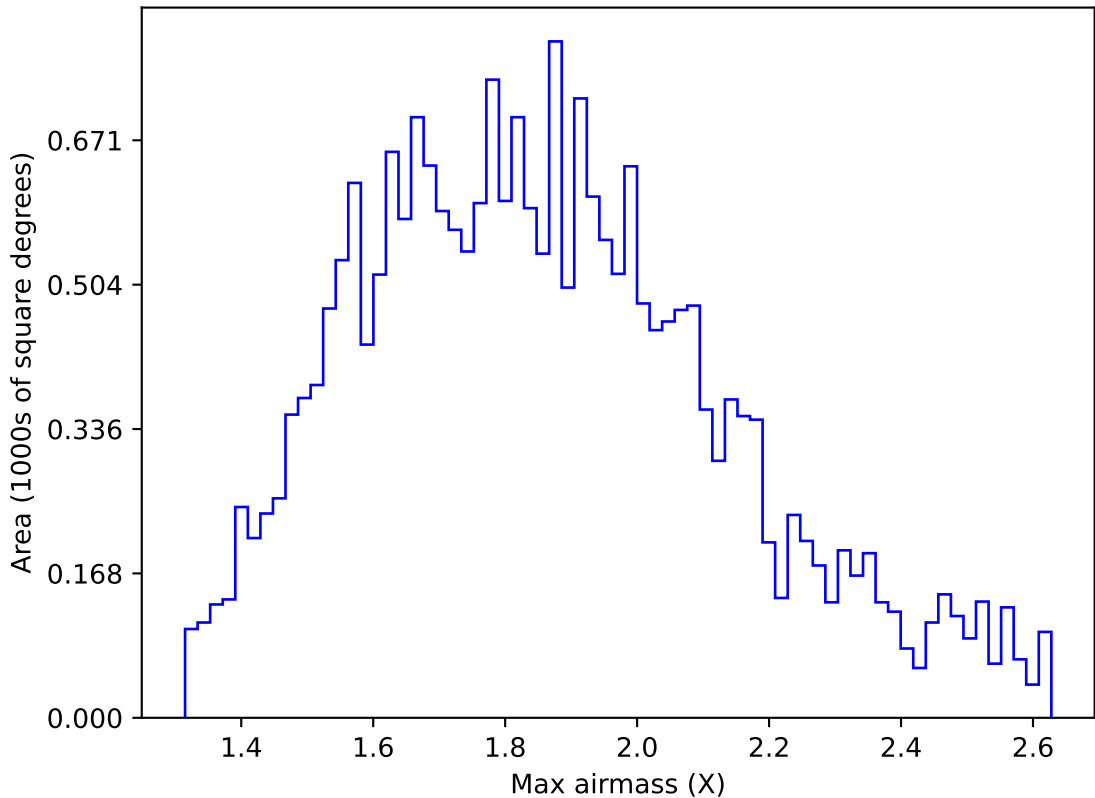
internal_u_expt27_nscale1.5v3.4_10yrs All sky u band: Max airmass
