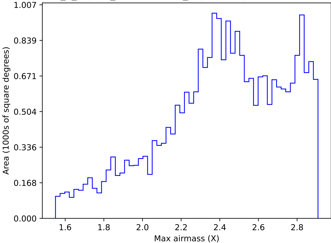
internal_u_expt27_nscale1.5v3.4_10yrs All sky i band: Max airmass
