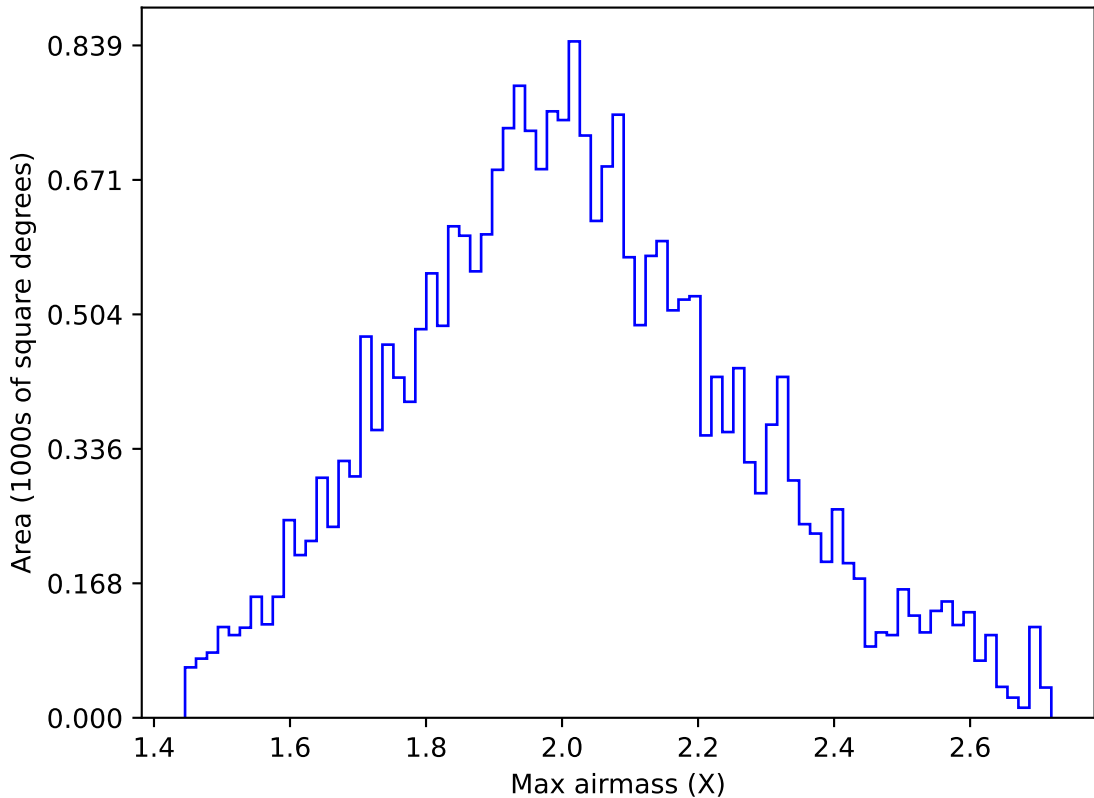
internal_u_expt27_nscale1.5v3.4_10yrs All sky g band: Max airmass
