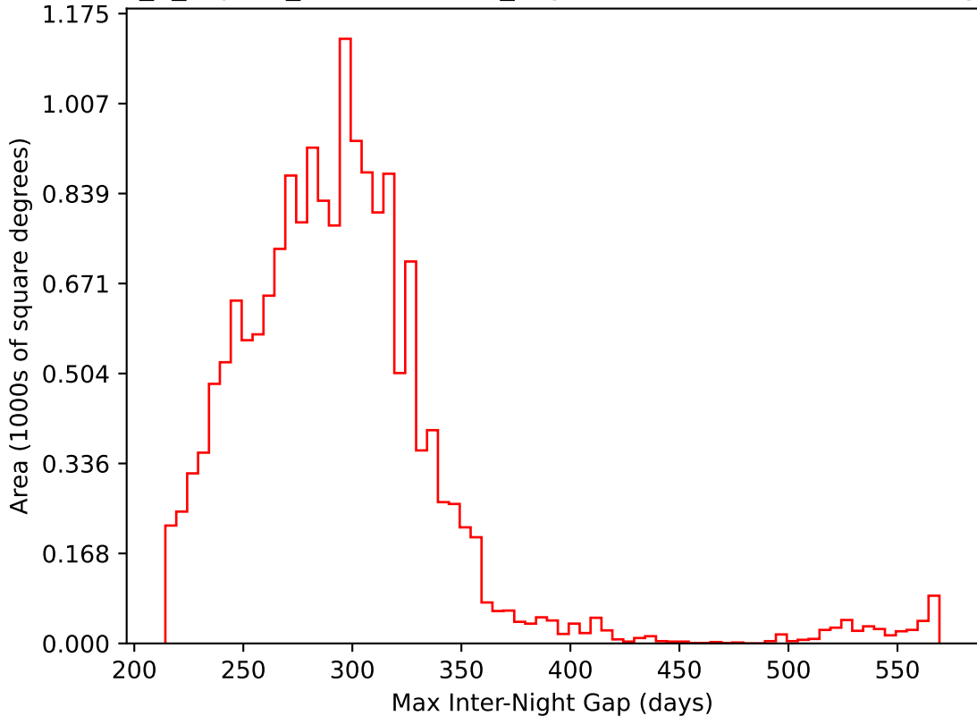
internal_u_expt27_nscale1.5v3.4_10yrs WFD i band: Max Inter-Night Gap
