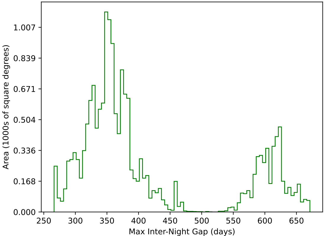
internal_u_expt27_nscale1.5v3.4_10yrs WFD g band: Max Inter-Night Gap
