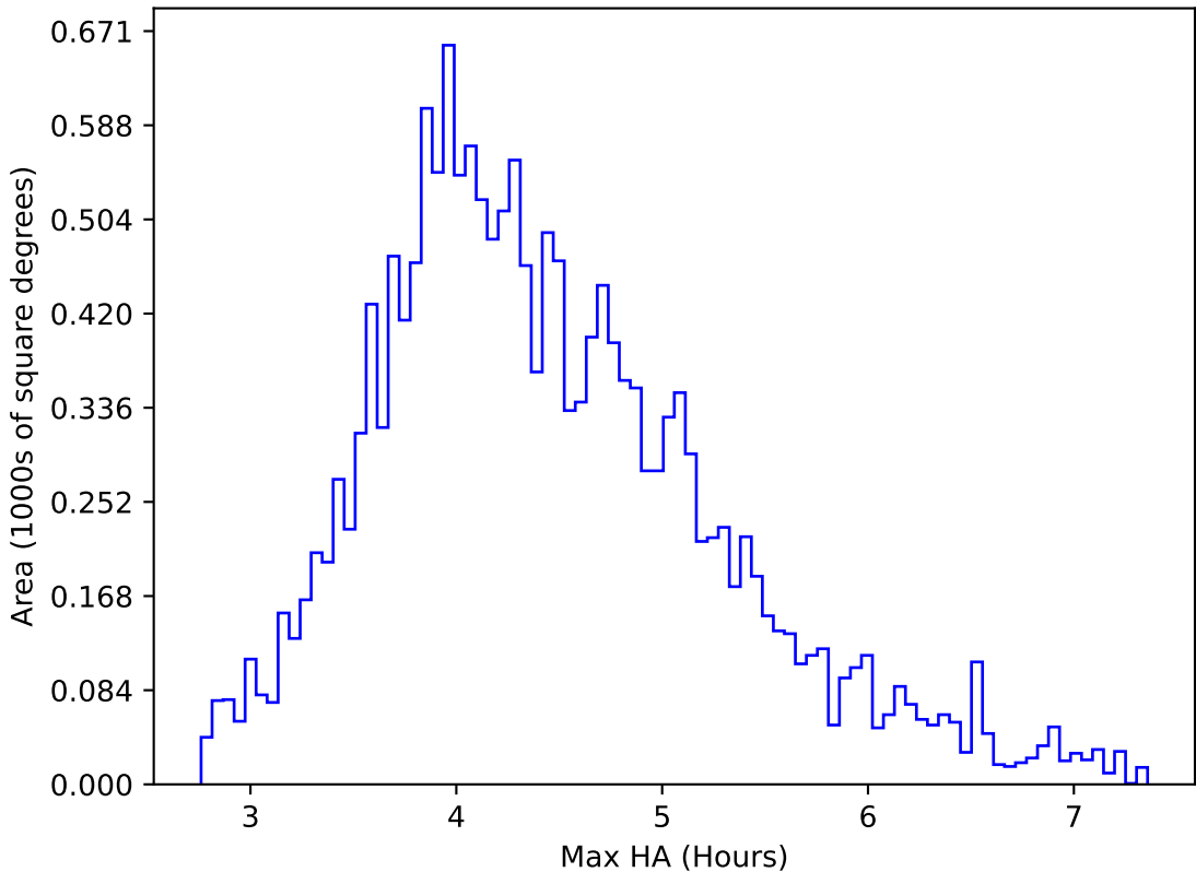
internal_u_expt27_nscale1.5v3.4_10yrs WFD r band: Max HA
