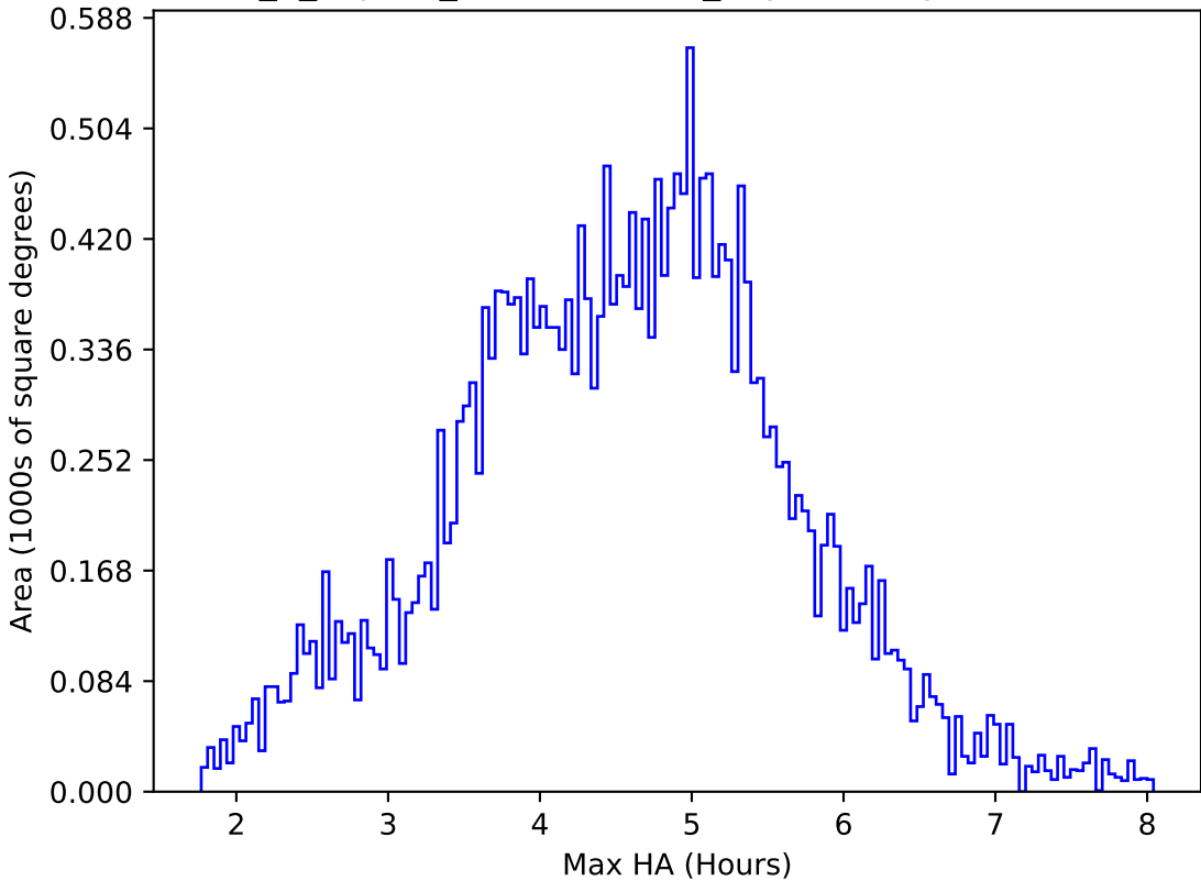
internal_u_expt27_nscale1.5v3.4_10yrs All sky z band: Max HA
