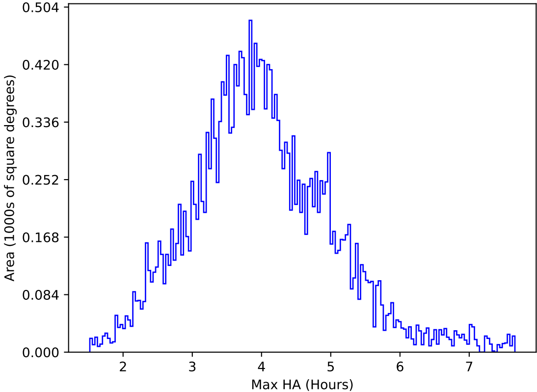
internal_u_expt27_nscale1.5v3.4_10yrs All sky u band: Max HA
