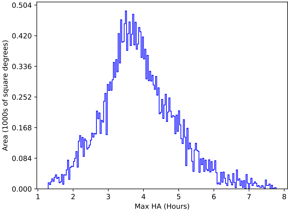
internal_u_expt27_nscale1.5v3.4_10yrs All sky g band: Max HA
