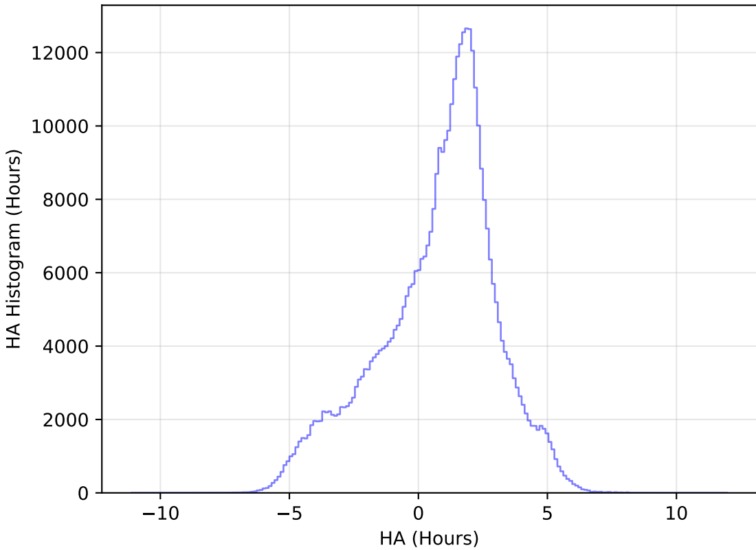
internal_u_expt27_nscale1.5v3.4_10yrs WFD z band: HA Histogram
