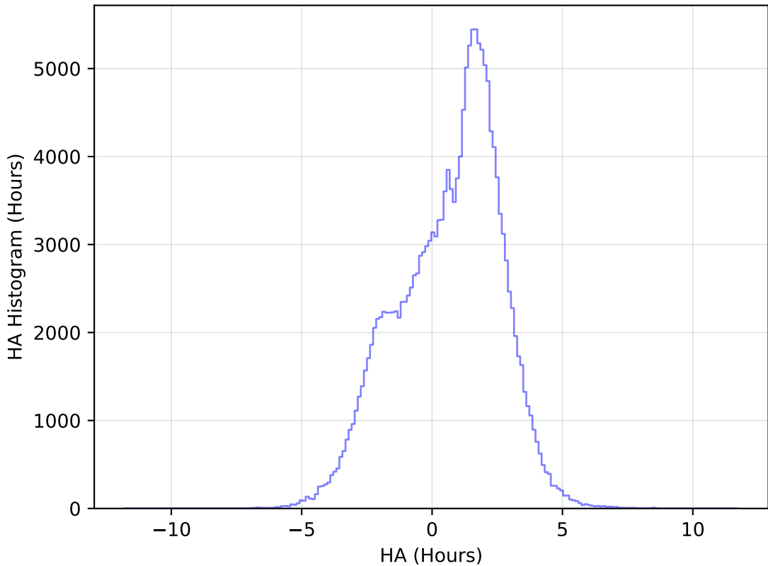
internal_u_expt27_nscale1.5v3.4_10yrs WFD u band: HA Histogram
