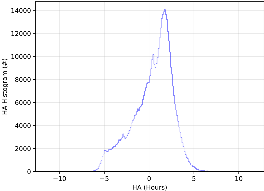
internal_u_expt27_nscale1.5v3.4_10yrs WFD r band: HA Histogram
