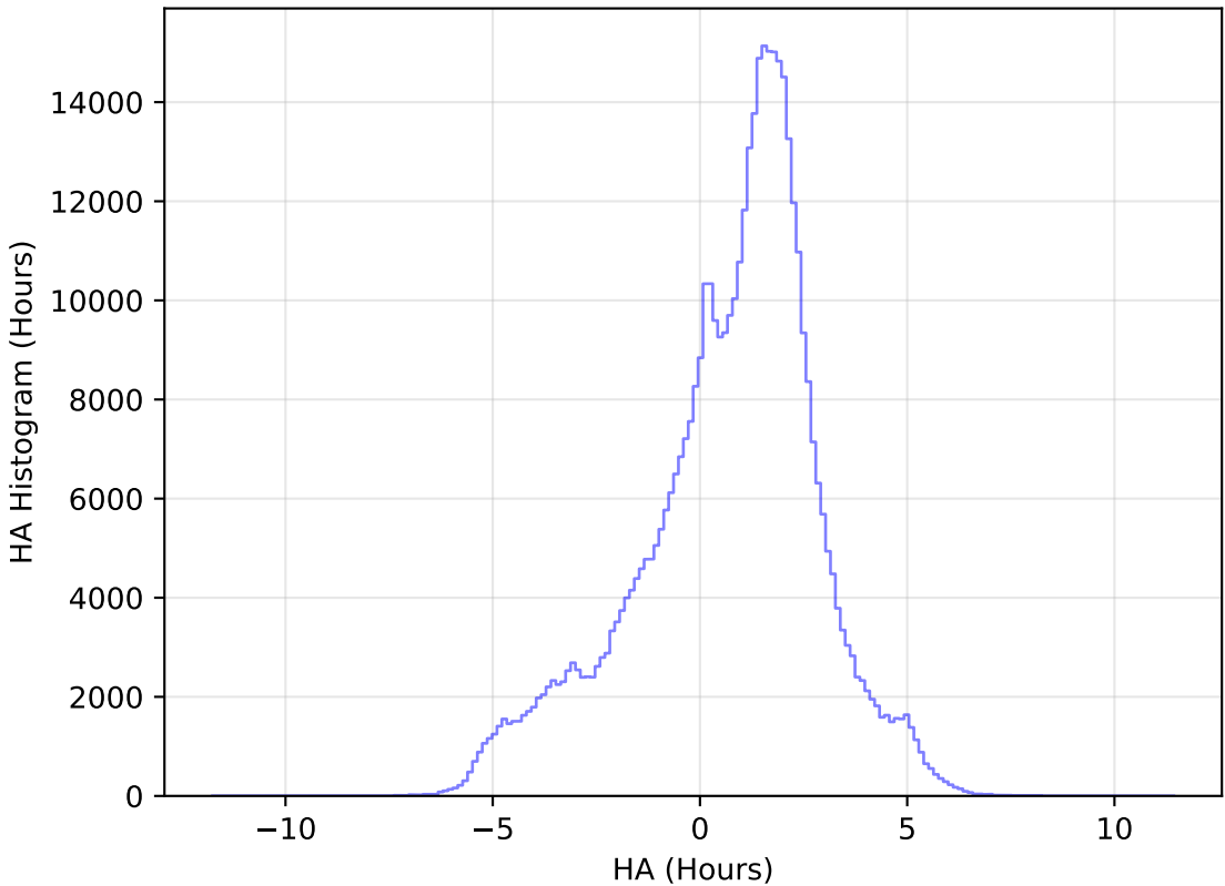
internal_u_expt27_nscale1.5v3.4_10yrs WFD i band: HA Histogram
