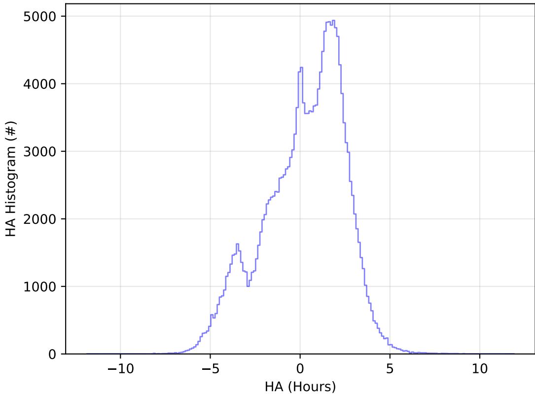
internal_u_expt27_nscale1.5v3.4_10yrs WFD g band: HA Histogram
