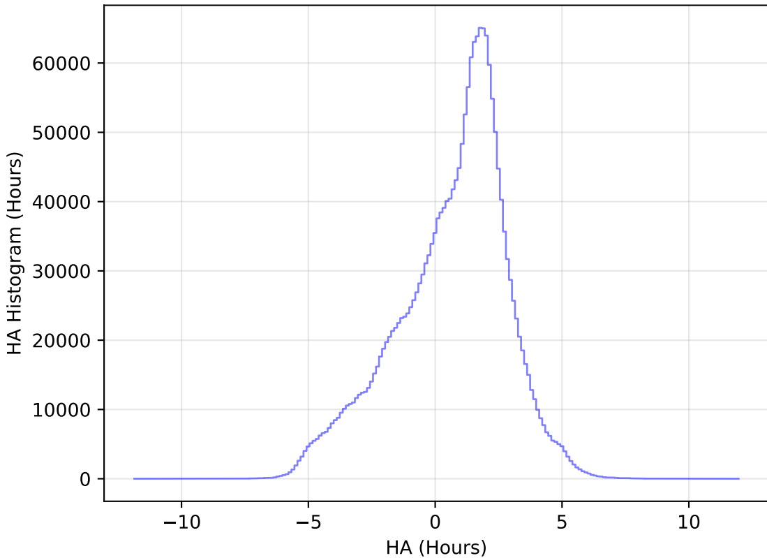
internal_u_expt27_nscale1.5v3.4_10yrs WFD all bands: HA Histogram
