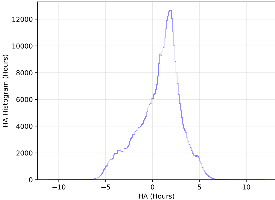
internal_u_expt27_nscale1.5v3.4_10yrs All sky z band: HA Histogram
