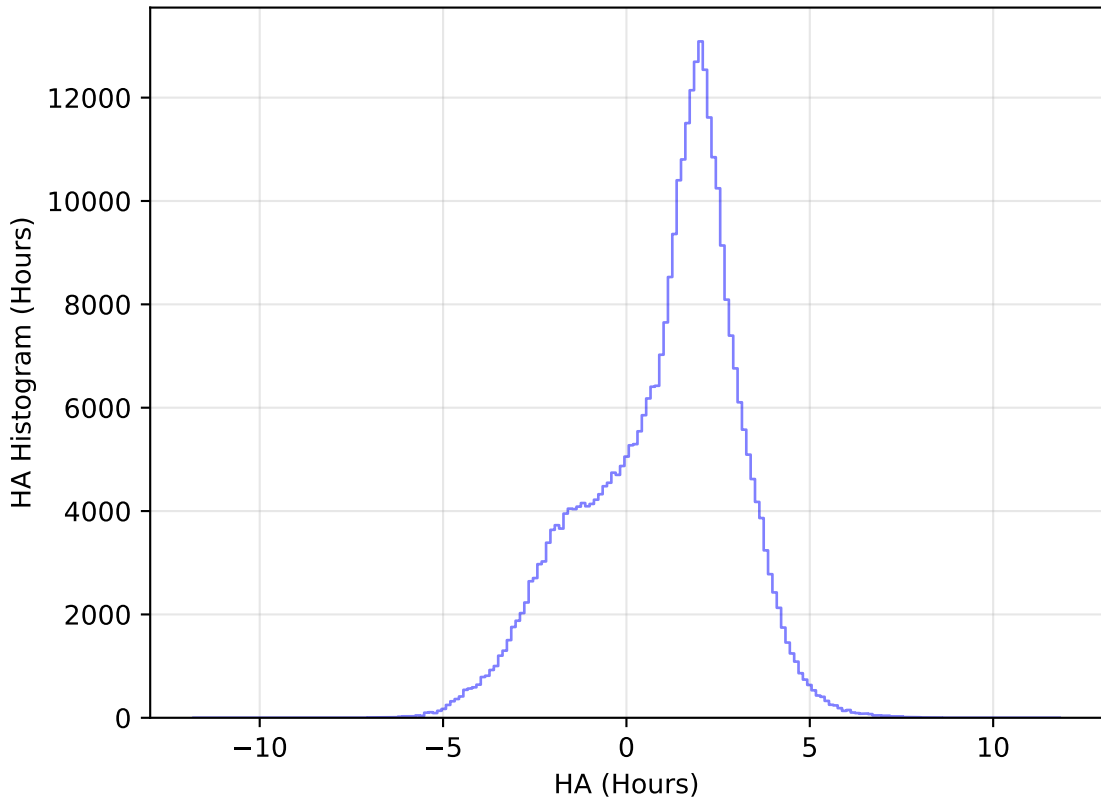
internal_u_expt27_nscale1.5v3.4_10yrs All sky y band: HA Histogram
