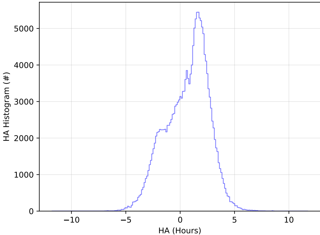
internal_u_expt27_nscale1.5v3.4_10yrs All sky u band: HA Histogram
