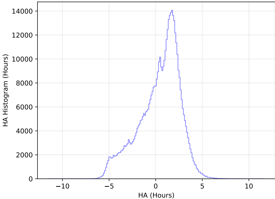
internal_u_expt27_nscale1.5v3.4_10yrs All sky r band: HA Histogram
