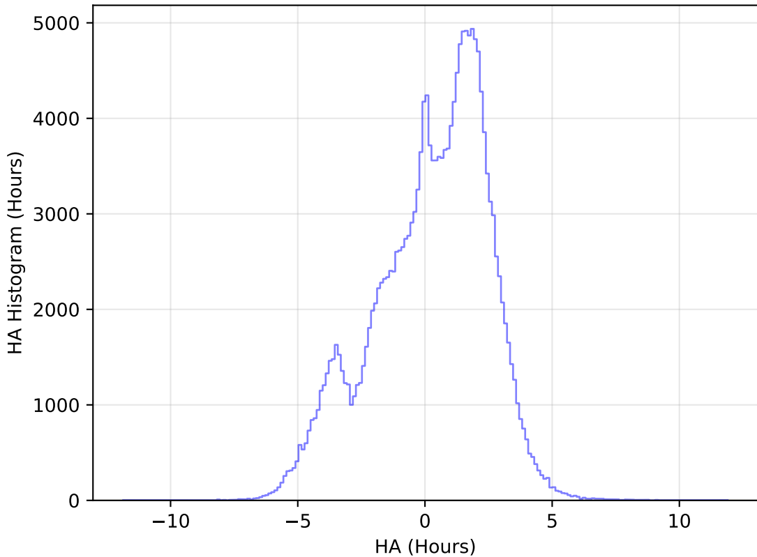
internal_u_expt27_nscale1.5v3.4_10yrs All sky g band: HA Histogram
