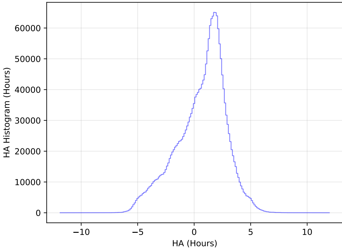
internal_u_expt27_nscale1.5v3.4_10yrs All sky all bands: HA Histogram
