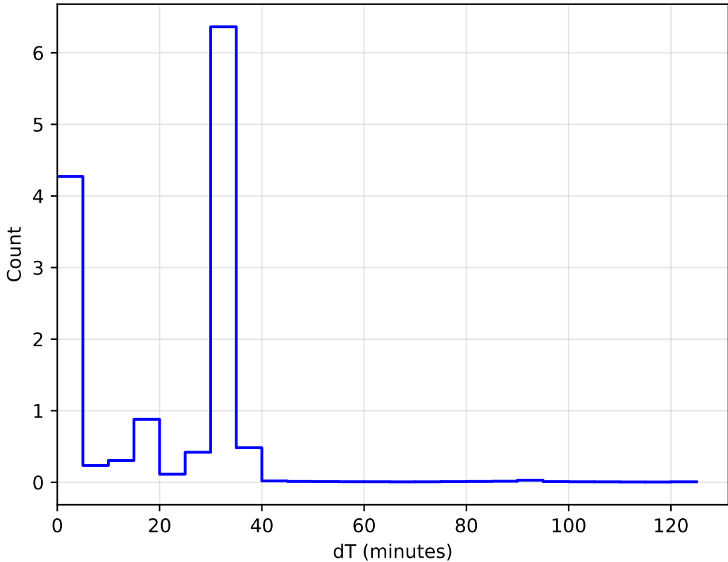
internal_u_expt27_nscale1.5v3.4_10yrs All sky: DeltaT Histogram
