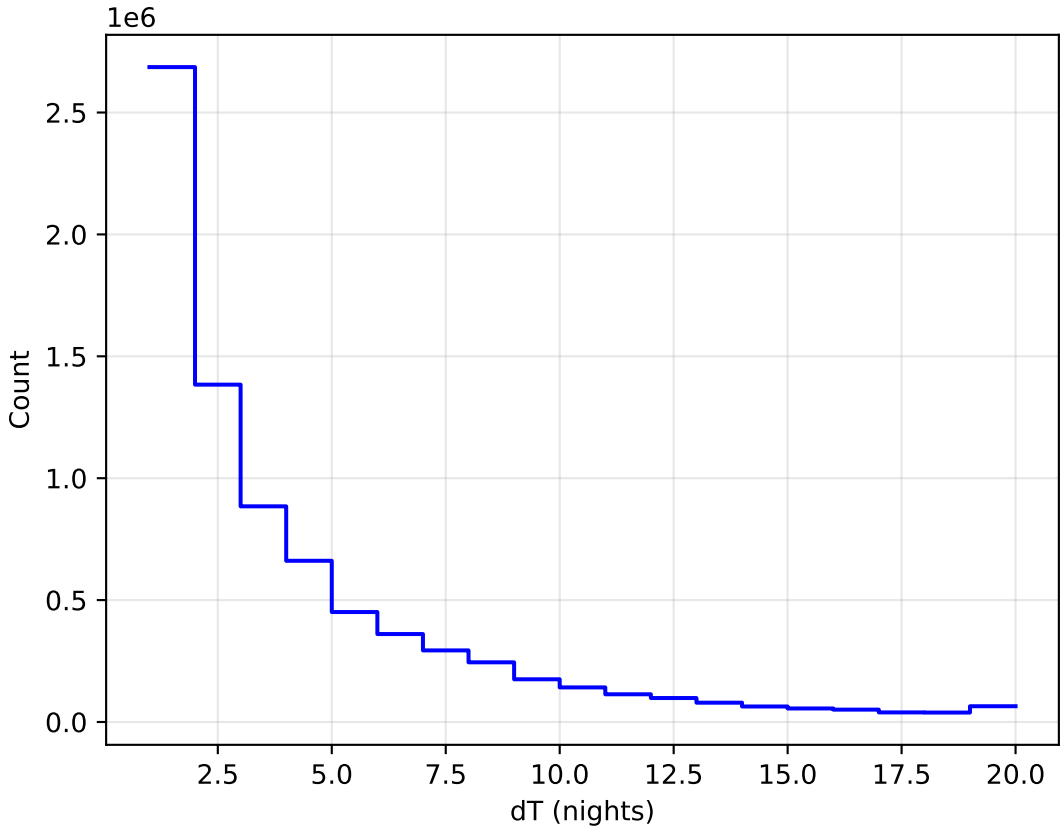
internal_u_expt27_nscale1.5v3.4_10yrs WFD all bands: DeltaNight Histogram
