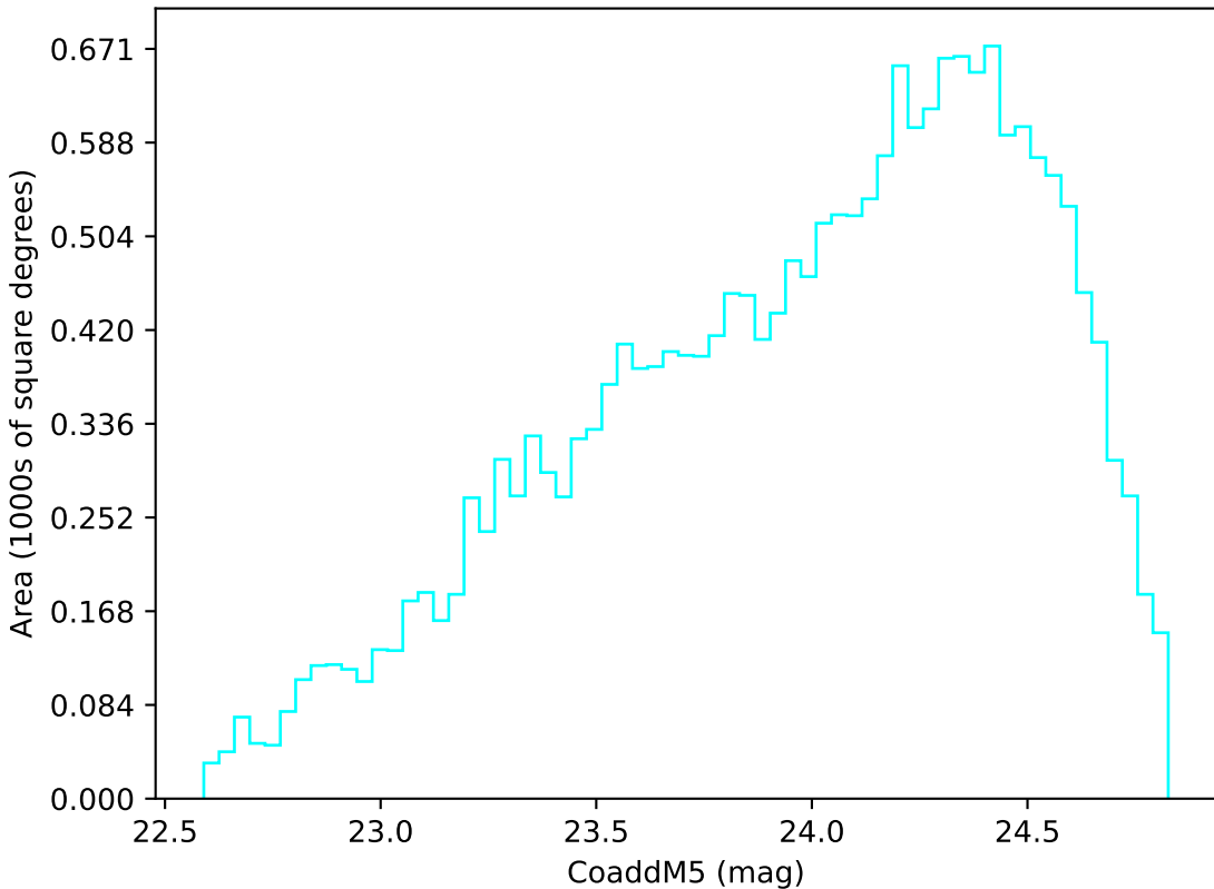
internal_u_expt27_nscale1.5v3.4_10yrs Yr 3-4 u band: CoaddM5
