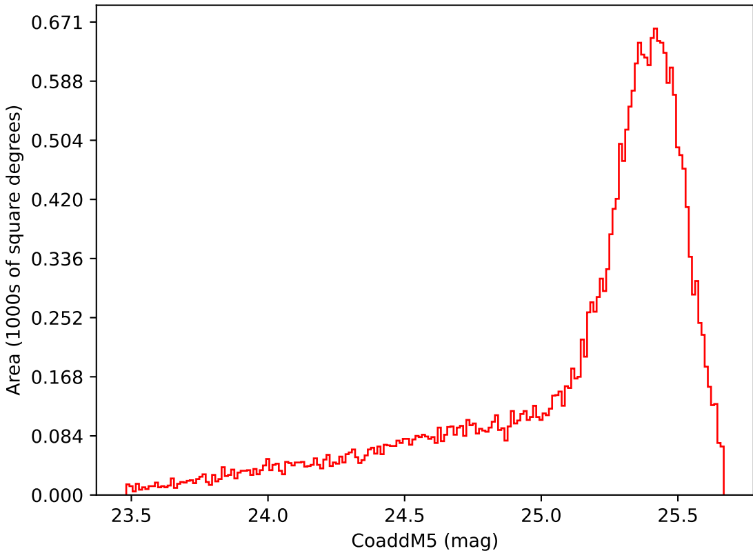
internal_u_expt27_nscale1.5v3.4_10yrs Yr 1 i band: CoaddM5
