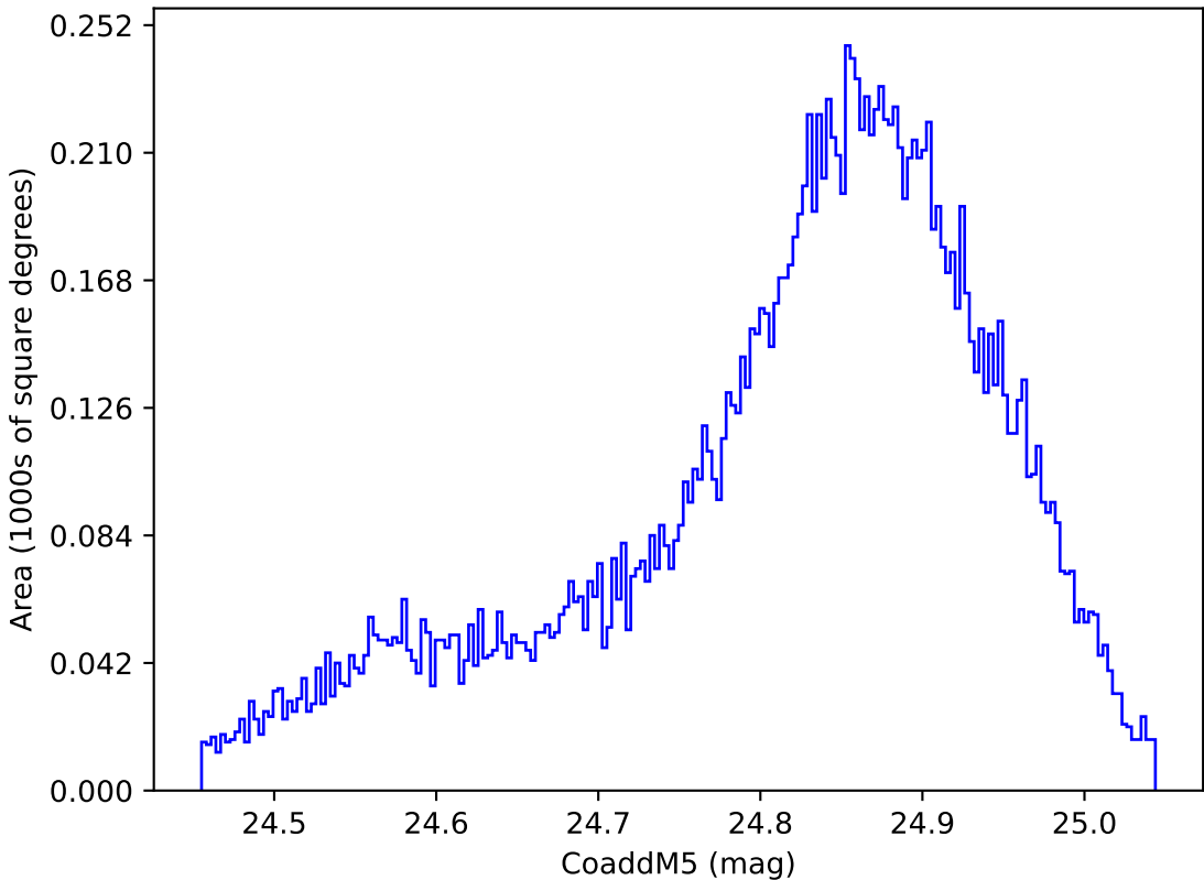
internal_u_expt27_nscale1.5v3.4_10yrs WFD y band: CoaddM5
