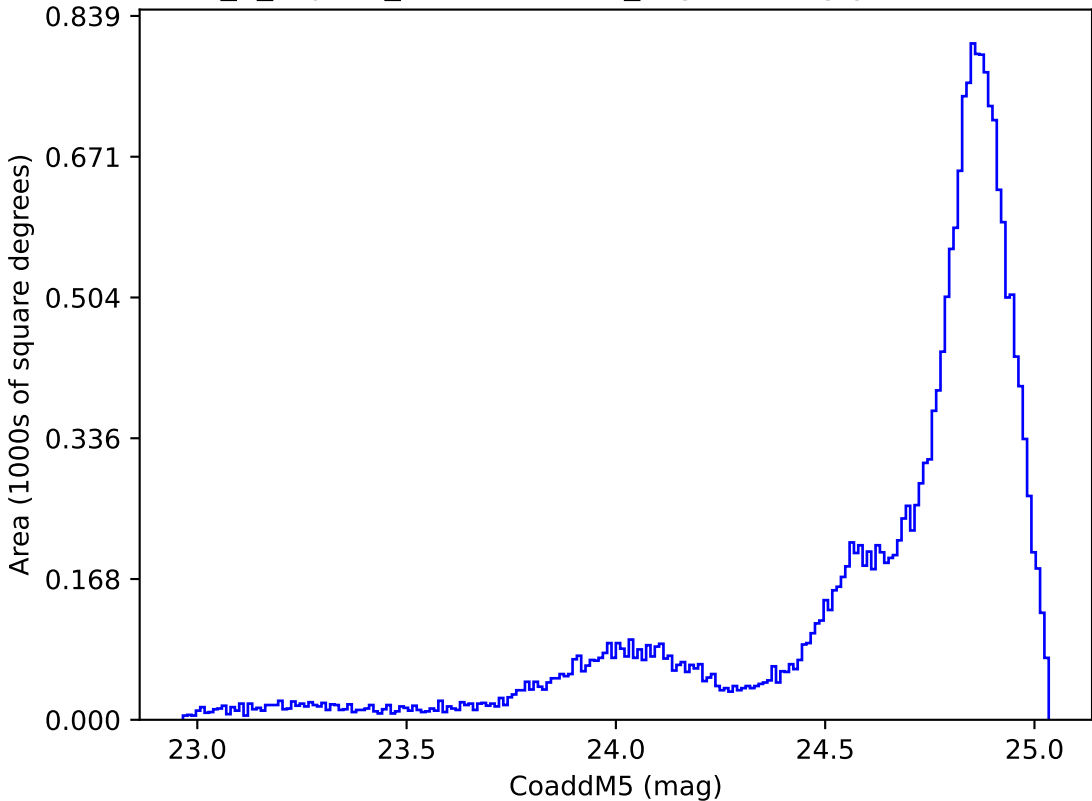
internal_u_expt27_nscale1.5v3.4_10yrs All sky y band: CoaddM5
